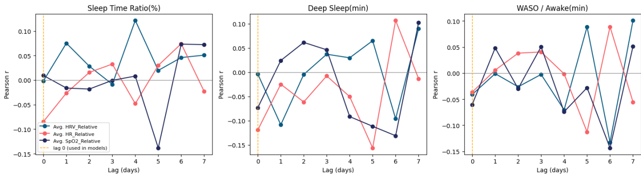
Figure 5. Lagged Pearson correlations between relative HRV, heart rate and SpO 2 and each sleep outcome (Sleep Time Ratio, Deep Sleep, WASO) at lags of 0–7 days. The orange dashed line marks lag 0, i.e. the same-day values used as predictors in the models. All correlations are weak and none reach statistical significance.
